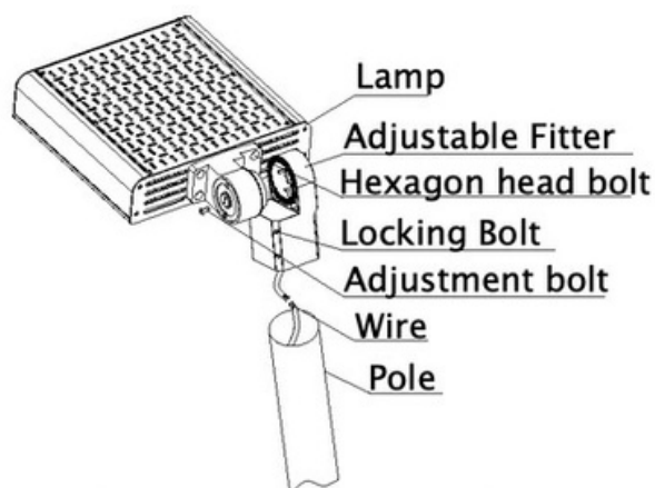
Fig1 (Exploded Views)
